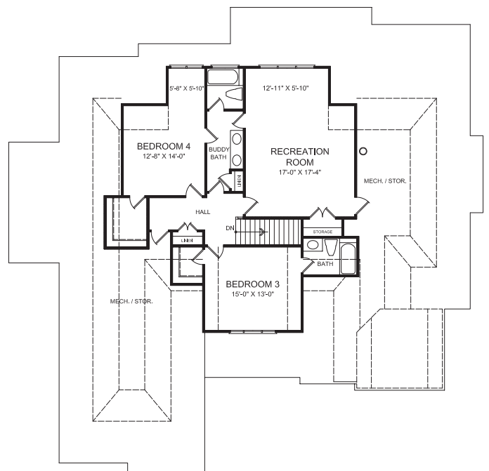
SECOND FLOOR
